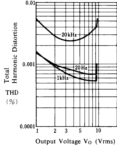
Total Harmonic Distortion vs. Output Voltage ( V^+/V^- = \pm 15V , R_L = 10k\Omega , Gain = 20dB, T_a = 25^\circ C )
